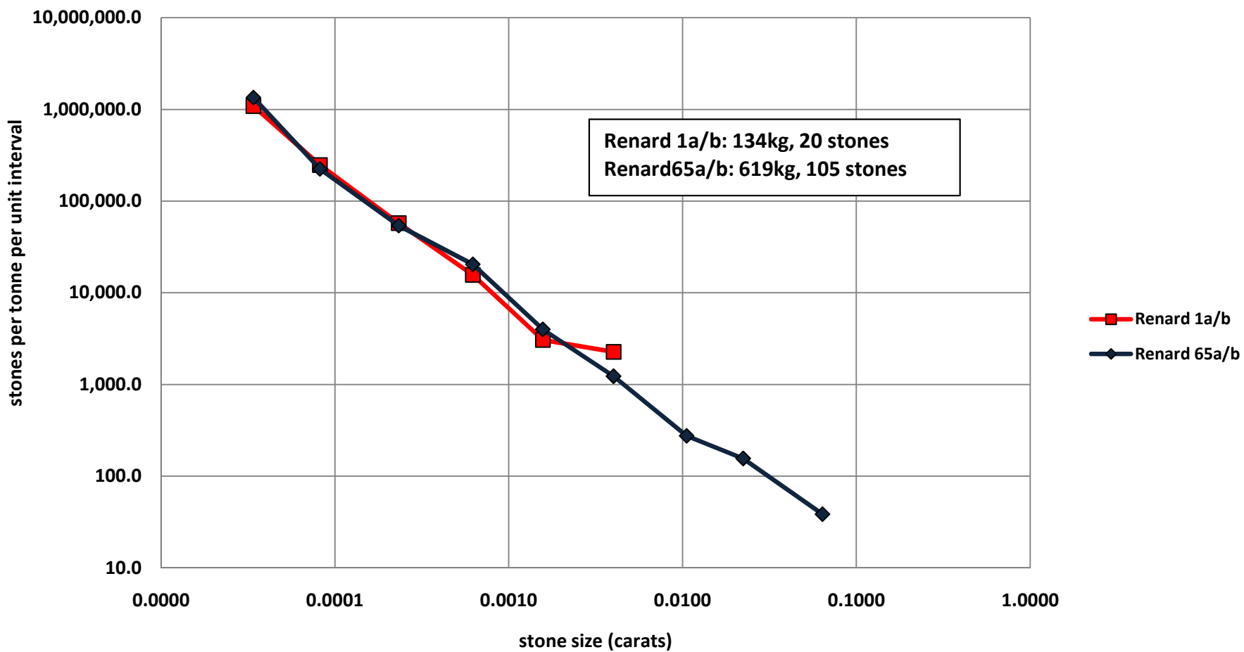
Renard 1 versus Renard 65 Microdiamond Spt_ui Plot
